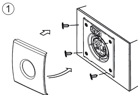
INSTALLATION MURALE
