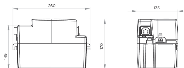
Dimensions (mm)
