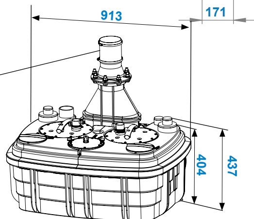
DISCHARGE PIPE CONNECTION DN 100
