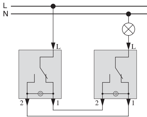
Two-way switch with locator light Mxx3x36-0000
