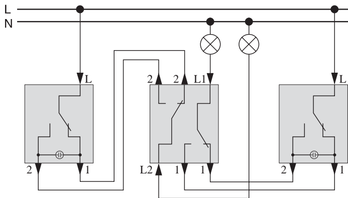
Two-way switch with locator light Mxx3x36-0000
