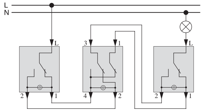
Two-way switch with locator light Mxx3x36-0000
